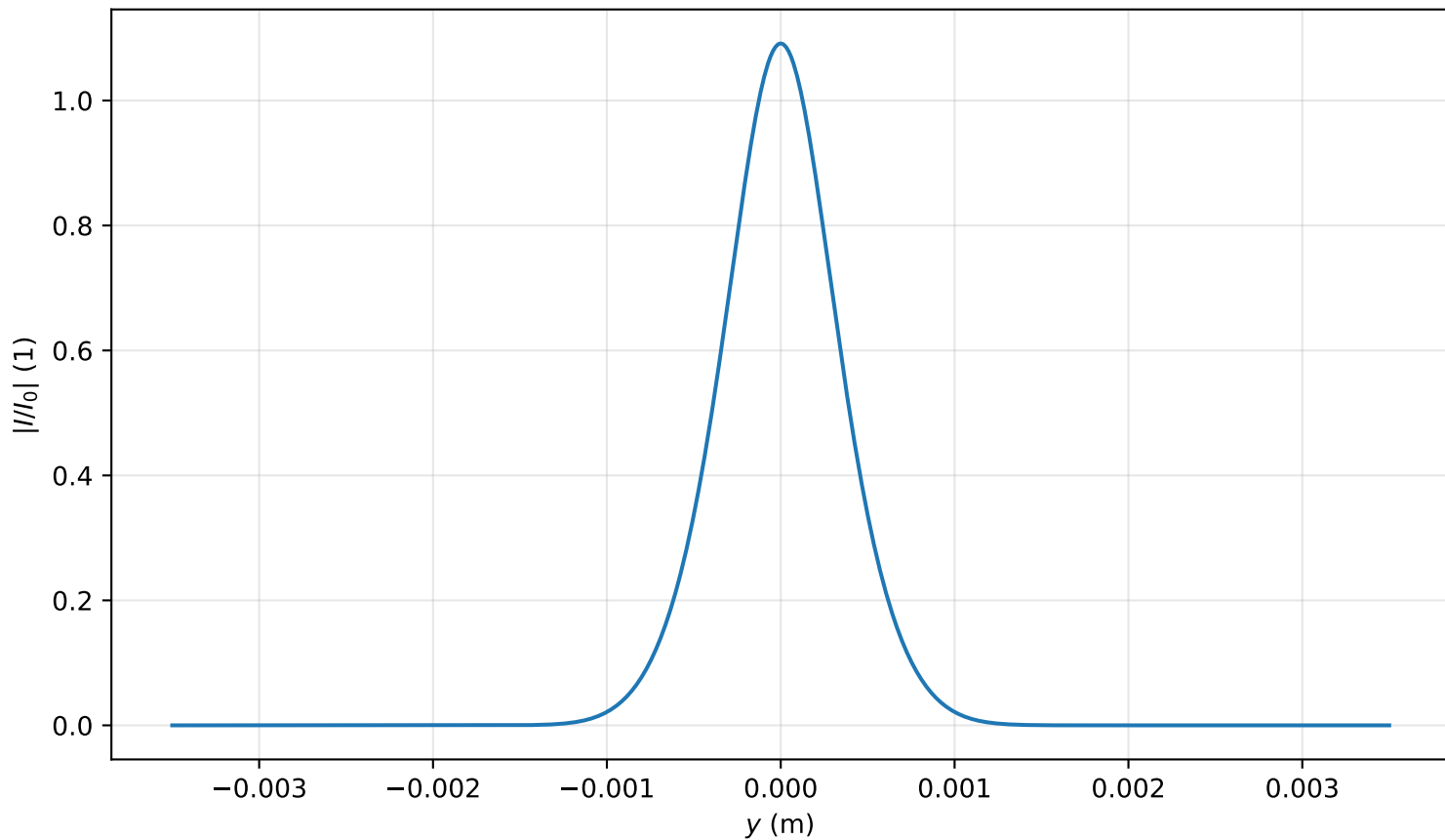
Intensity profile I(x = 0, y, z = 0.637)/I_0 , P_{in}=0.6P_{cr} , artificial time
